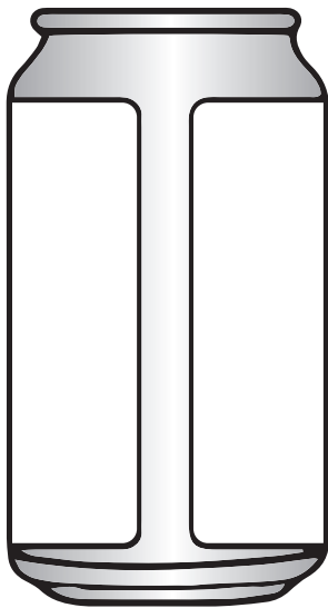
355ml die size 3.55" x 7.59" .3479" gap at the back
