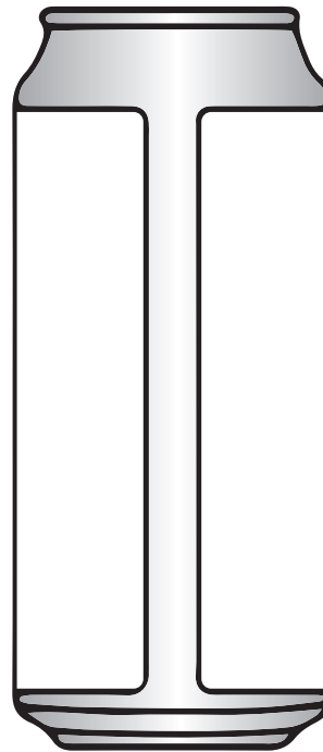
473ml die size 5" x 7.59" .3479" gap at the back
