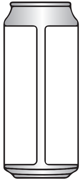
473ml die size 5" x 7.9375" .25" gap at the back
